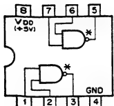
TC40107BP (TOSHIBA) C-MOS NAND BUFFER/DRIVER WITH OPEN-DRAIN — TOP VIEW —
